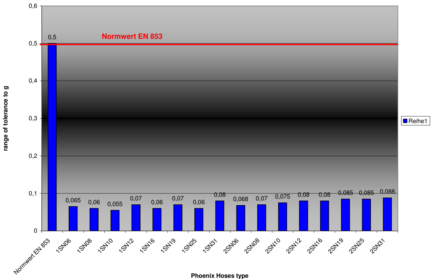
Phoenix Hydraulic Hoses 1SN and 2SN Standard -cover Abrasion Test according EN ISO 6945 Test-time 2005 to sep. 2008
